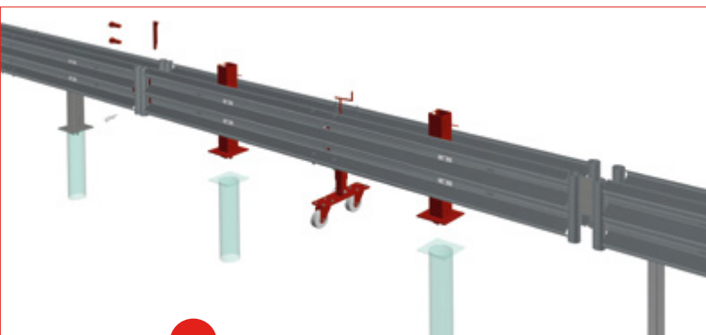
3. Disassembly and hang up the socket posts
