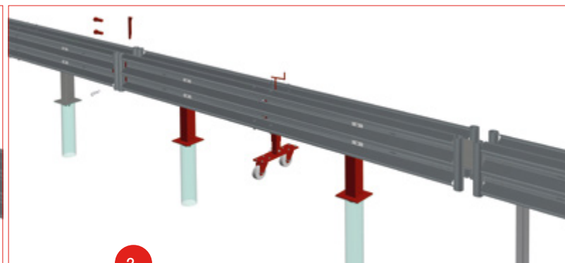
2. Disassembly of pin-wedge connection
